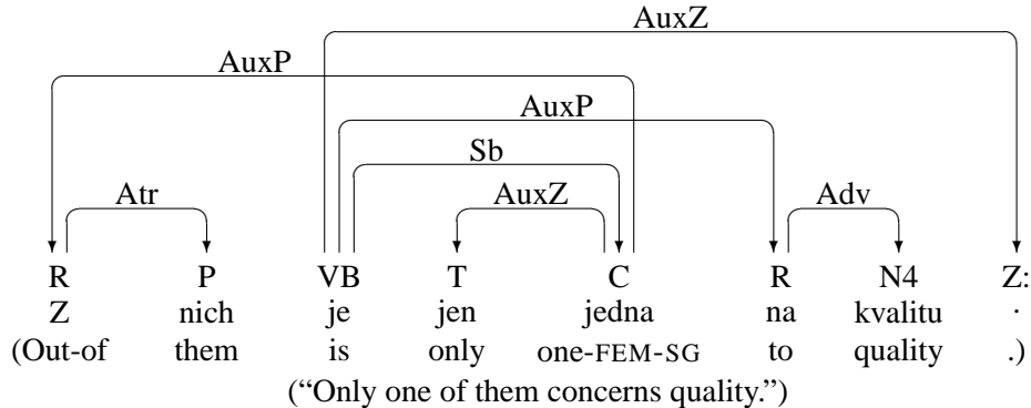
Figure 1: Dependency graph for Czech sentence from the Prague Dependency Treebank 1
